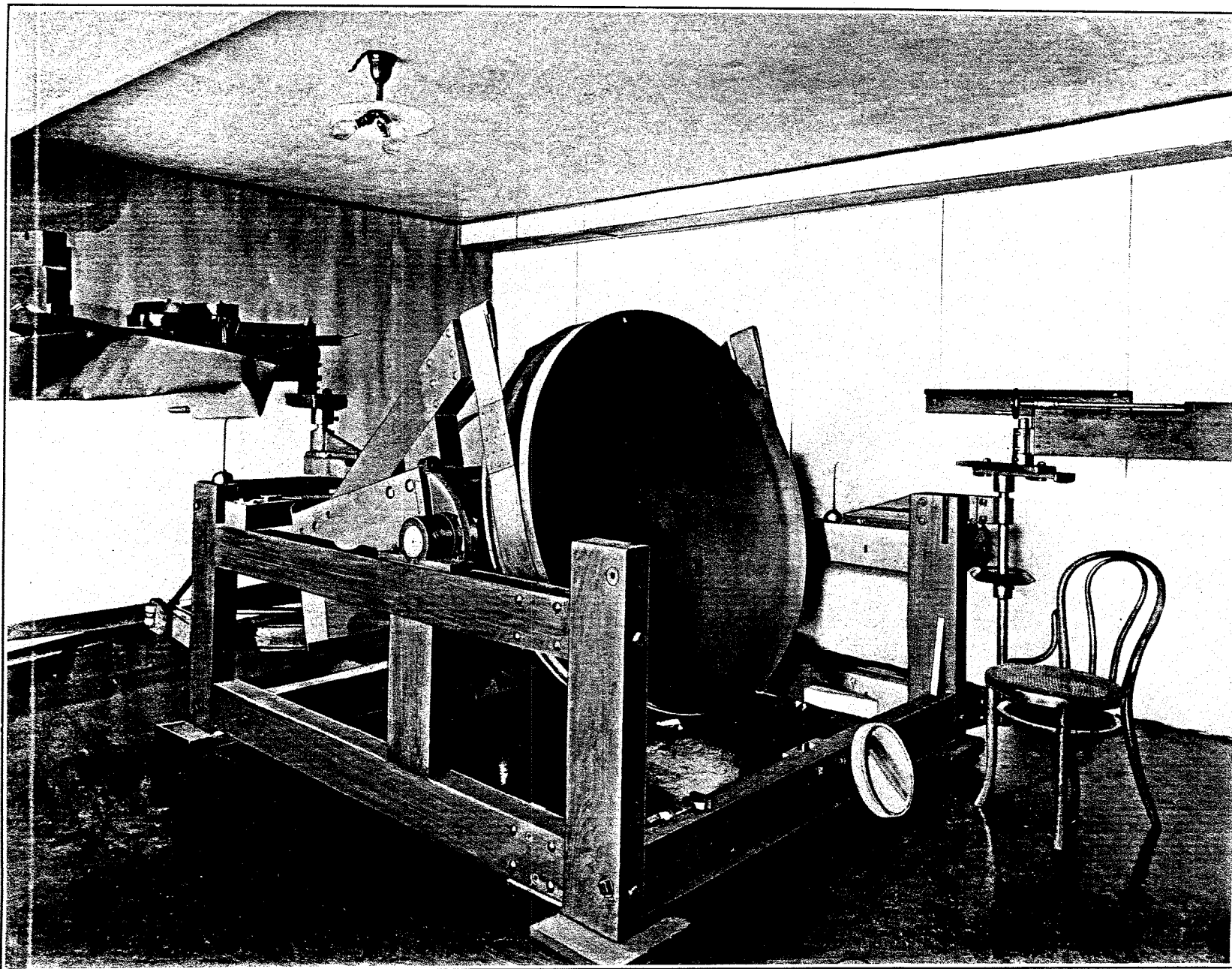
FIVE-FOOT MIRROR AND GRINDING MACHINE. SHOWING METHOD OF TIPPING GLASS ON EDGE FOR TESTING.
