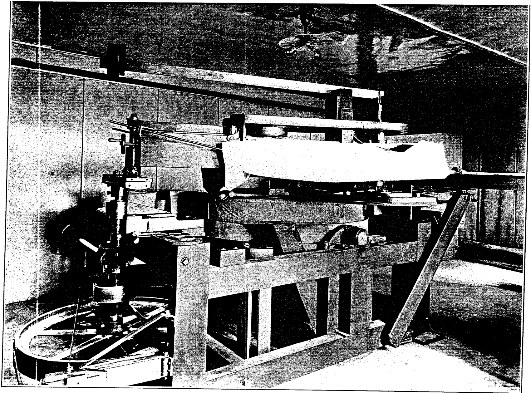
FIVE-FOOT MIRROR AND GRINDING MACHINE. SHOWING HALF-SIZE GRINDING TOOL SUSPENDED ON MAIN ARM.
