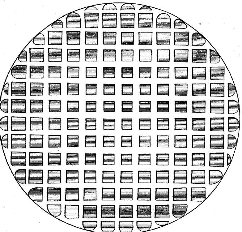
FIG. 6. CONVEXING POLISHING TOOL FOR FIGURING PLANE MIRROR.
