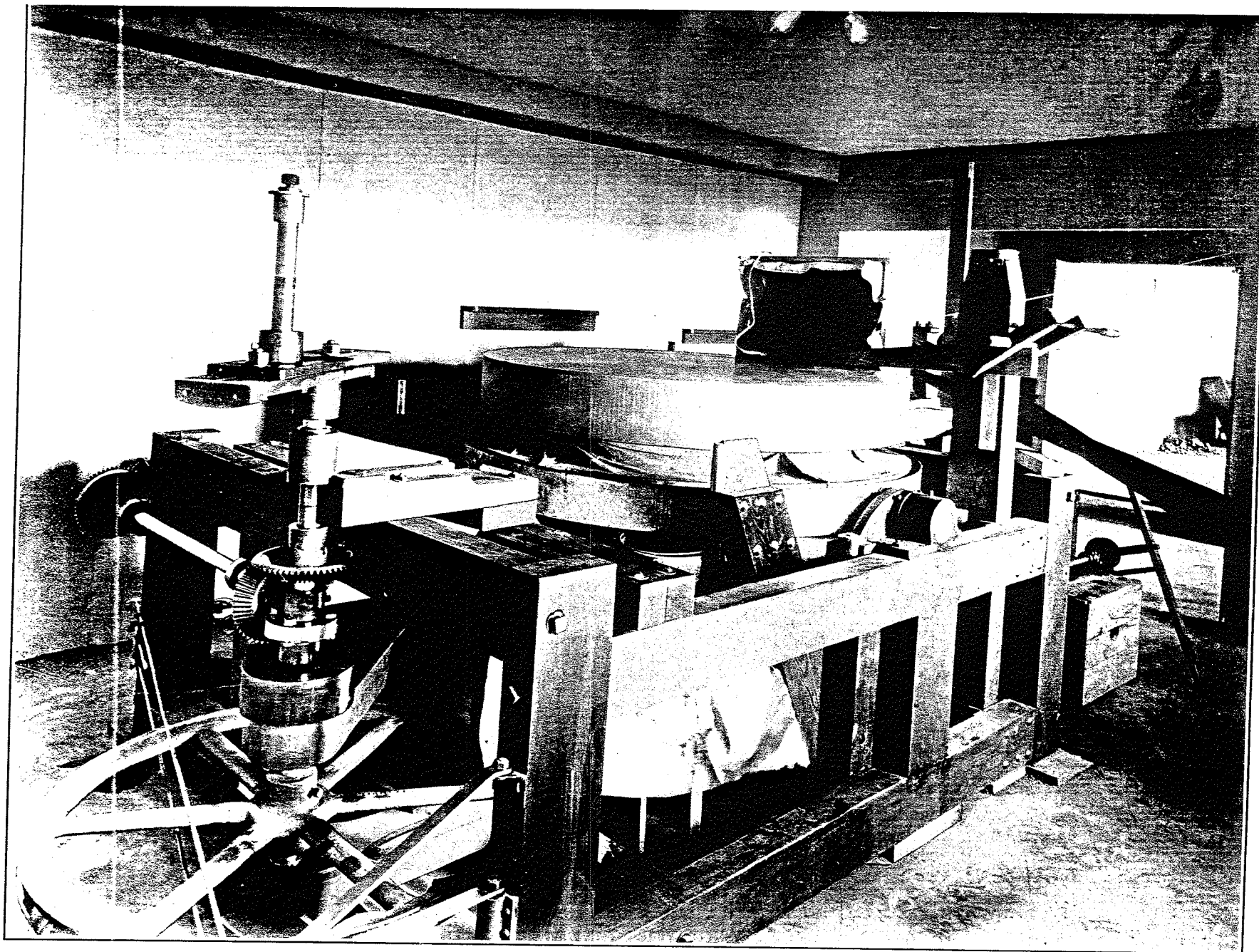
FIVE-FOOT MIRROR AND GRINDING MACHINE. METHOD OF GRINDING EDGE OF GLASS.
