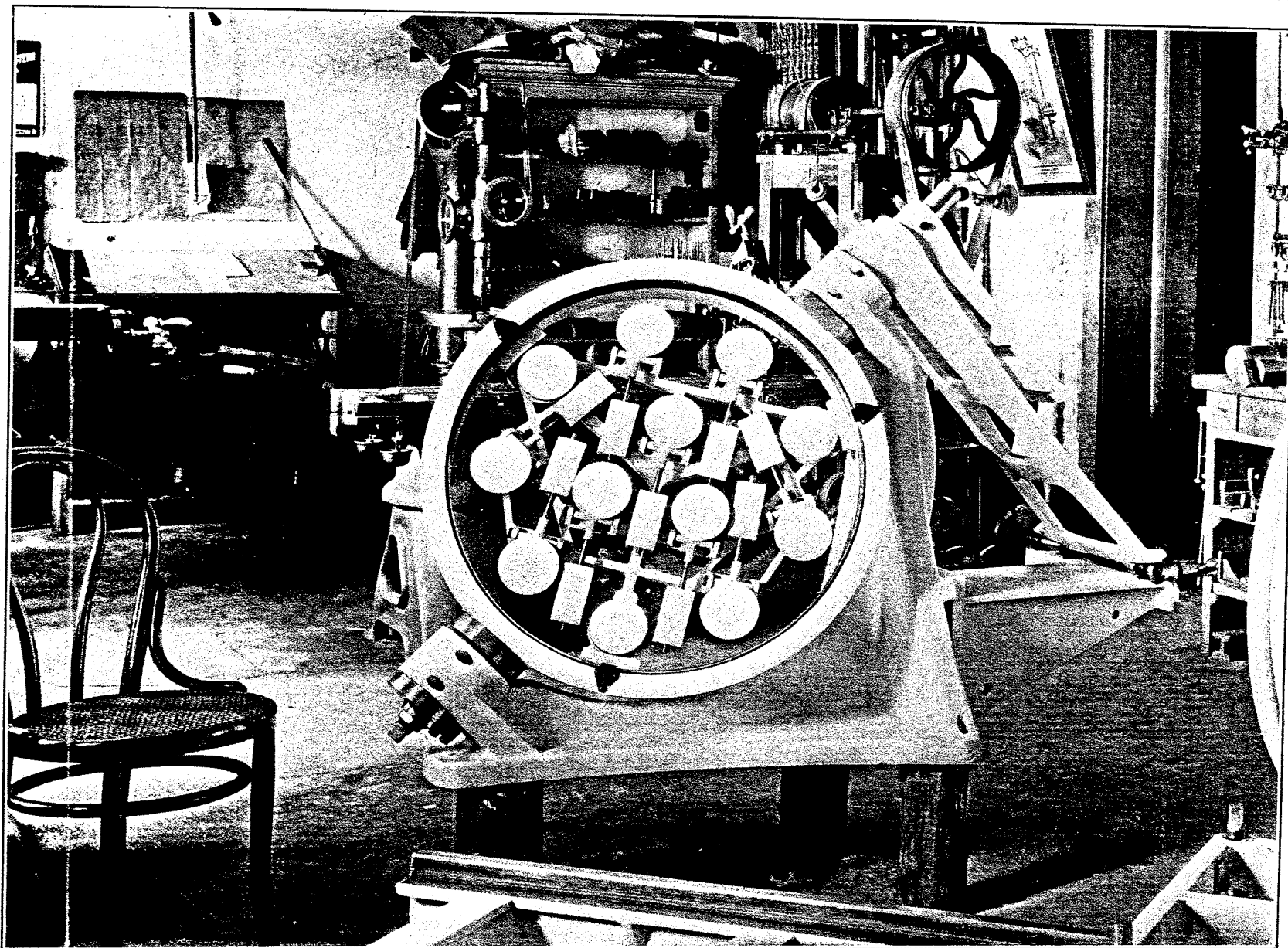
LARGE COELOSTAT WITH 30-INCH PLANE MIRROR. PLATES AND LEVERS FOR BACK-SUPPORT ARE SEEN THROUGH THE UNSILVERED GLASS.
