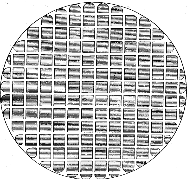
FIG. 4. NORMAL POLISHING TOOL.
