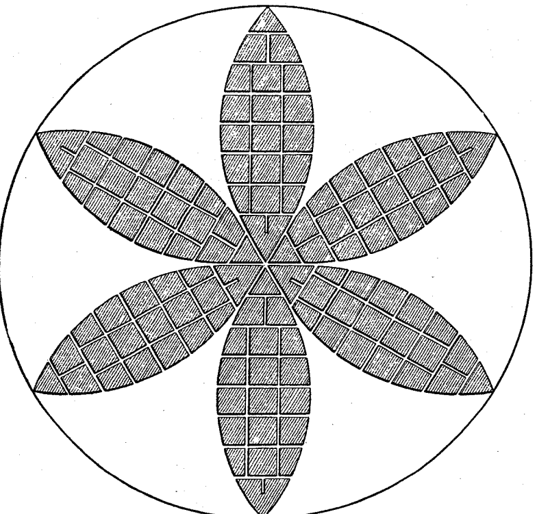
FIG. 13. FULL-SIZE POLISHING TOOL FOR PARABOLIZING.
