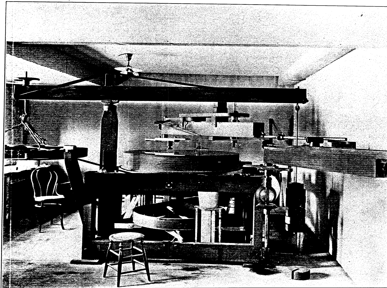
FIVE-FOOT MIRROR AND GRINDING MACHINE. SHOWING LEVER FOR HANDLING HEAVY GRINDING AND POLISHING TOOLS.
